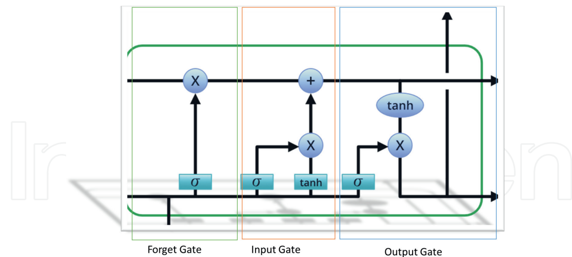
Figure 3. The basic structure of an LSTM model.
